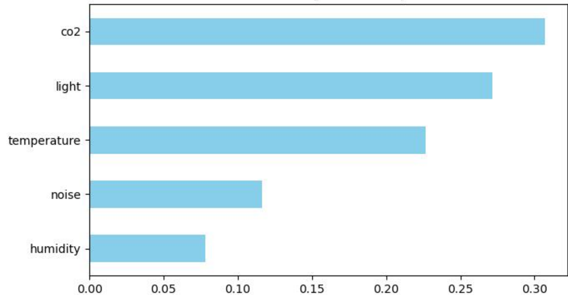
Gradient Boosting Feature Importance
